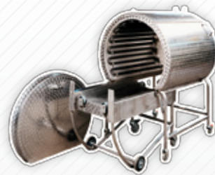
FK-DHDR Kombination in Edelstahl FK-DHDR combination unit in stainless steel
